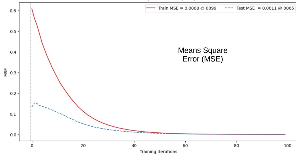
Estimator performance (MSE)
