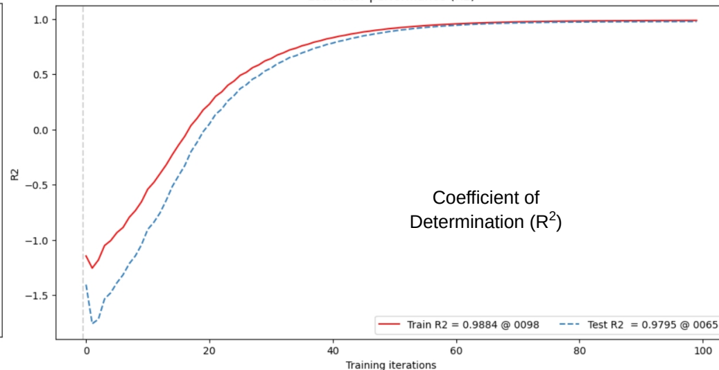
Estimator performance (R 2 )
